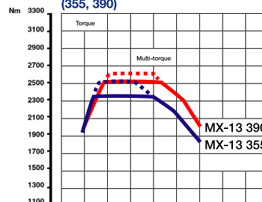
PACCAR MX-13 (355, 390)
